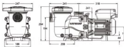
Dimensional Diagram
